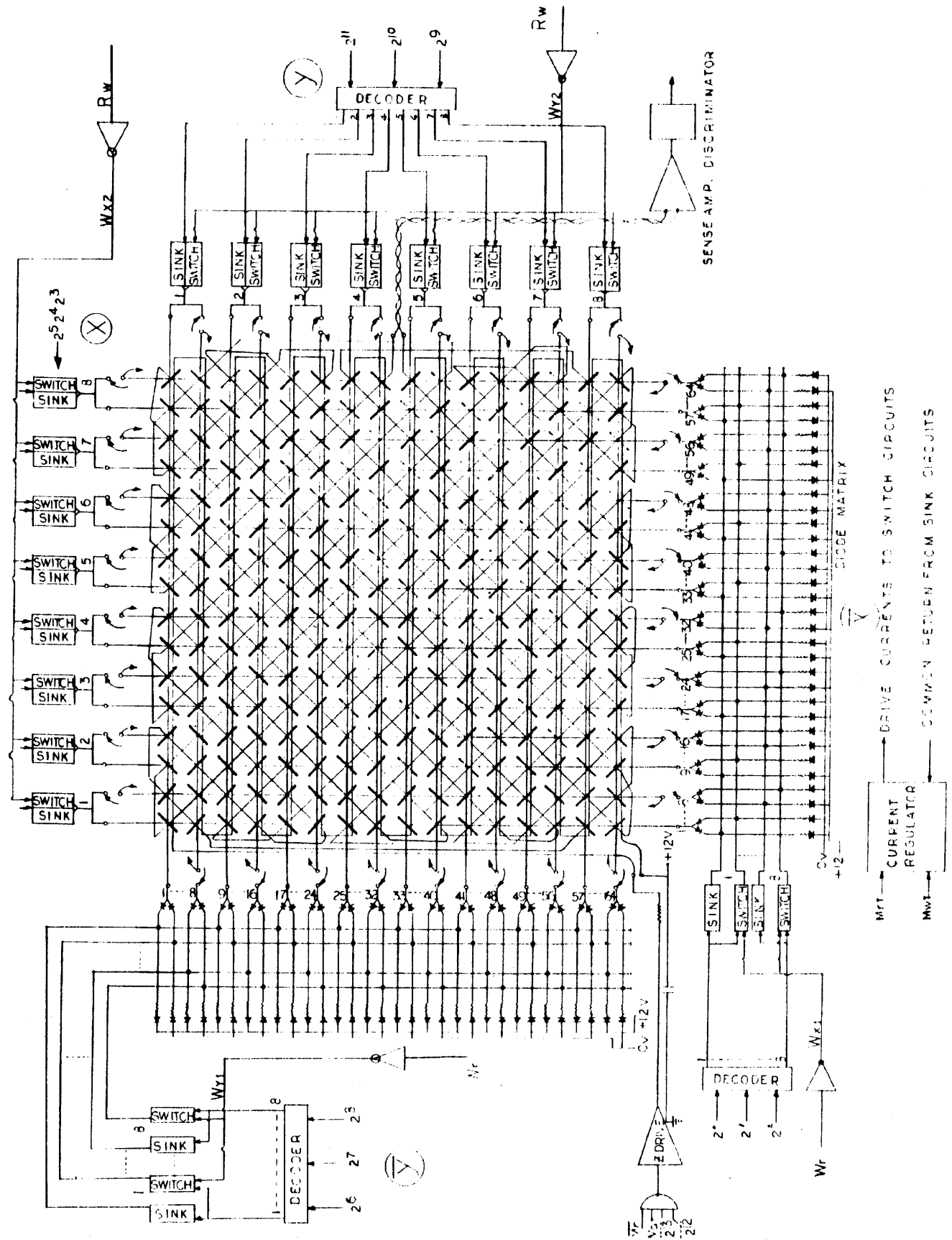
Figure 46. Memory Digit Plane Diagram
