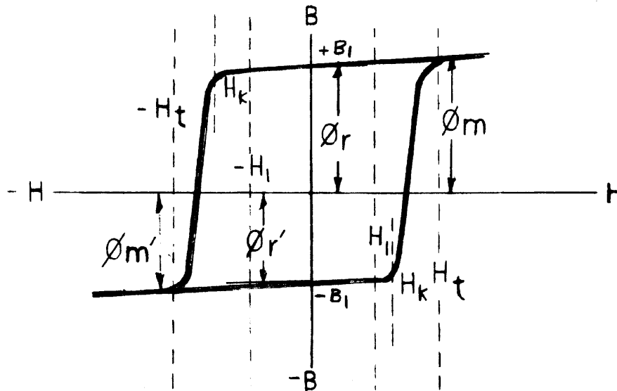
Figure 42 Hysteresis Loop
