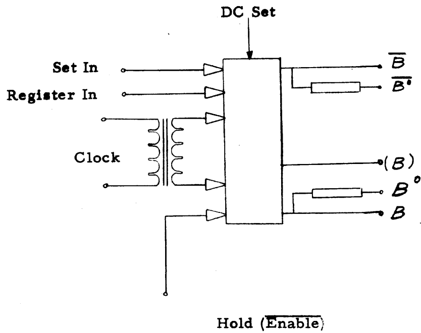
REPEATER FLIP-FLOP
